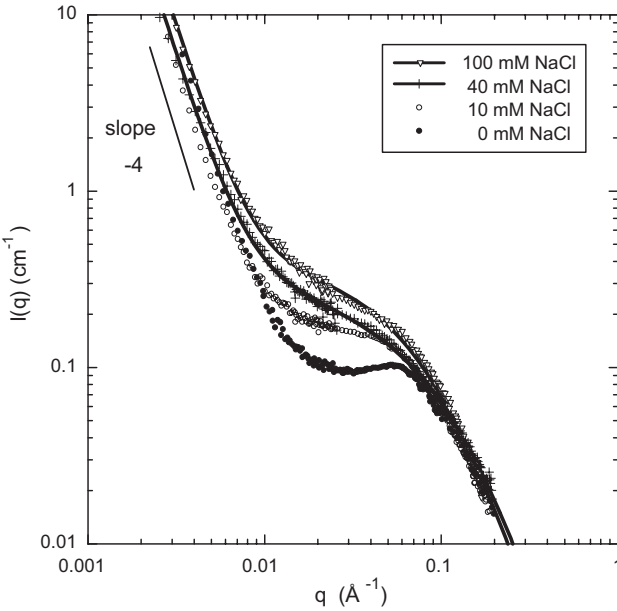
Figure 2. SANS intensity from DNA gels in equilibrium with solutions containing NaCl (0, 10, 40 and 100 mM). The continuous curves through the data points of the gels swollen in 40 mM NaCl and 100 mM NaCl solutions show the least squares fits to eq. 6 with F(q) = aq^{-4} .
